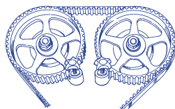
DUAL OVERHEAD CAM
