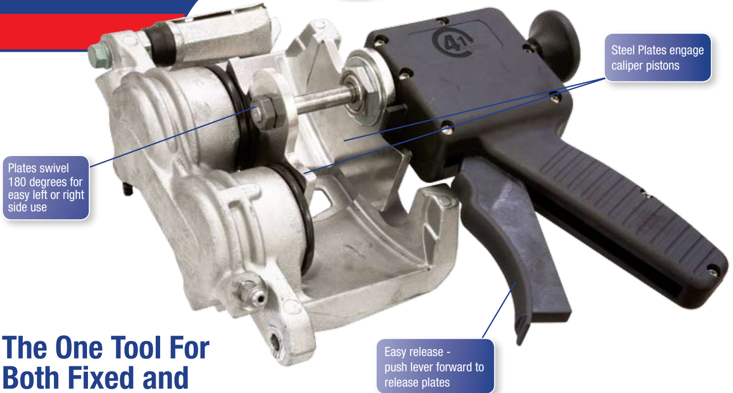
Single Floating Caliper
