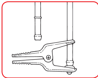
Fuel Line
