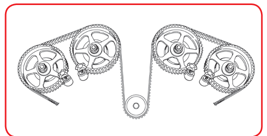
Quad Overhead Cam
