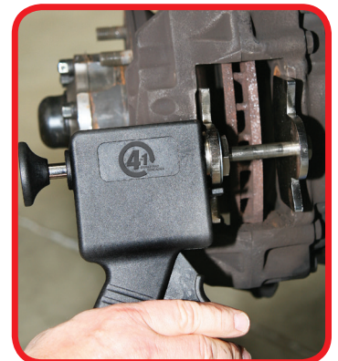
Twin Piston Fixed Caliper
