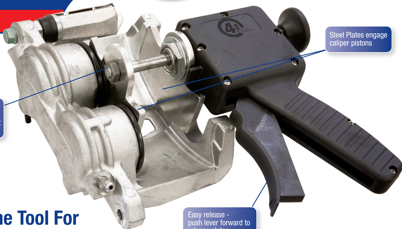
Single Floating Caliper
