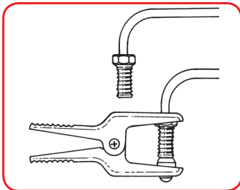
Flare Type Brake Line
