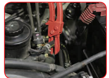
Small line clamp pliers in use
